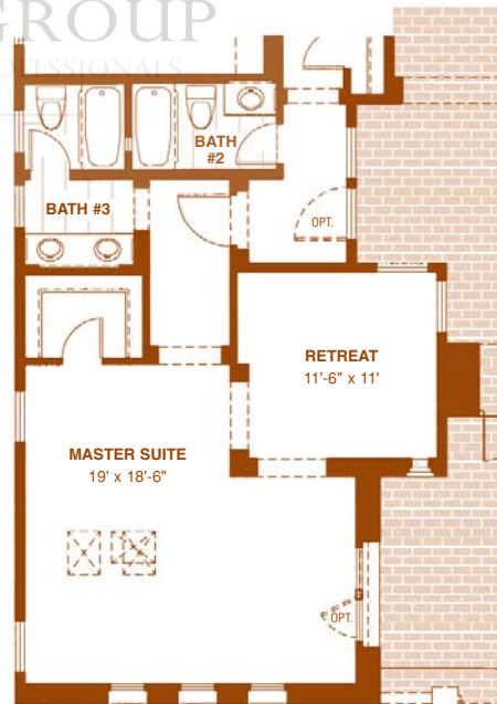
MASTER SUITE OPTION #3 (Elevation A Detail)
