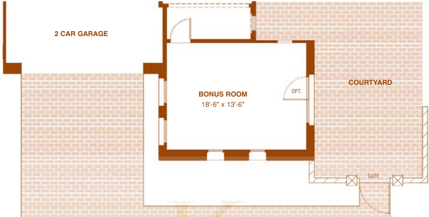
4' EXPANDED BONUS ROOM OPTION WITH 4' EXTENDED GARAGE
